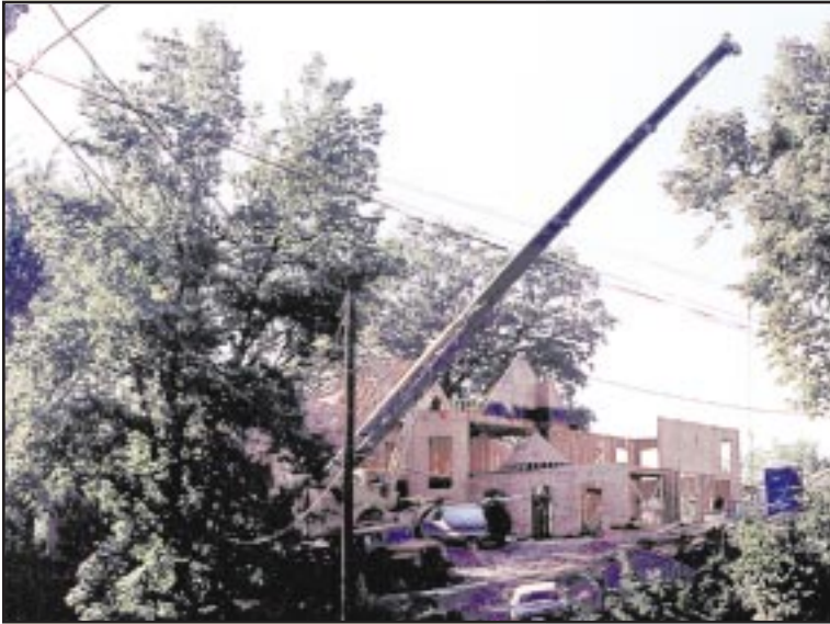
Operating a crane near overhead wires is very hazardous.
