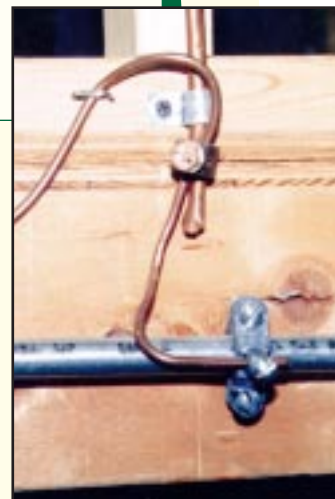
Install bonding jumpers around nonconductive material.
